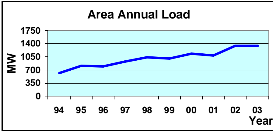
Figure A.2.21 – Area 21 Annual Load
