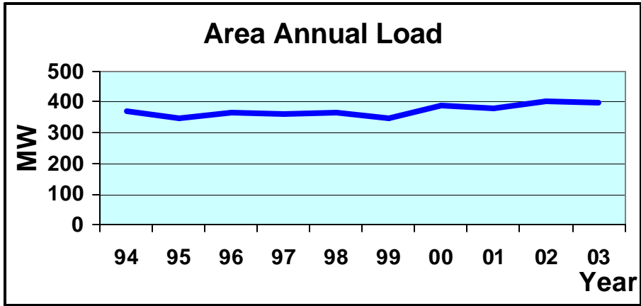
Figure A.2.9 – Area 9 Annual Load
