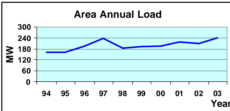
Figure A.2.8– Area 8 Annual Load
