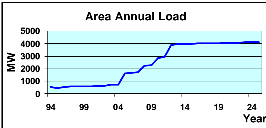
Figure A.2.29 – Area 19 Annual and Forecast Load
