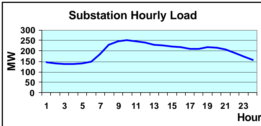
Figure A.3.7 – Substation 7 Hourly Load
