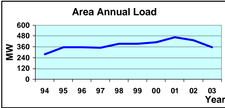
Figure A.2.3– Area 3 Annual Load
