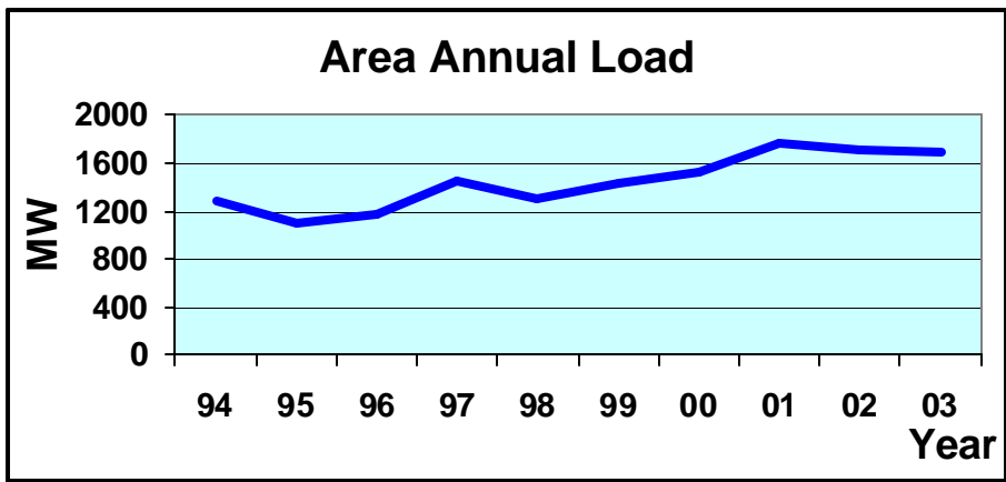
Figure A.2.20 – Area 20 Annual Load
