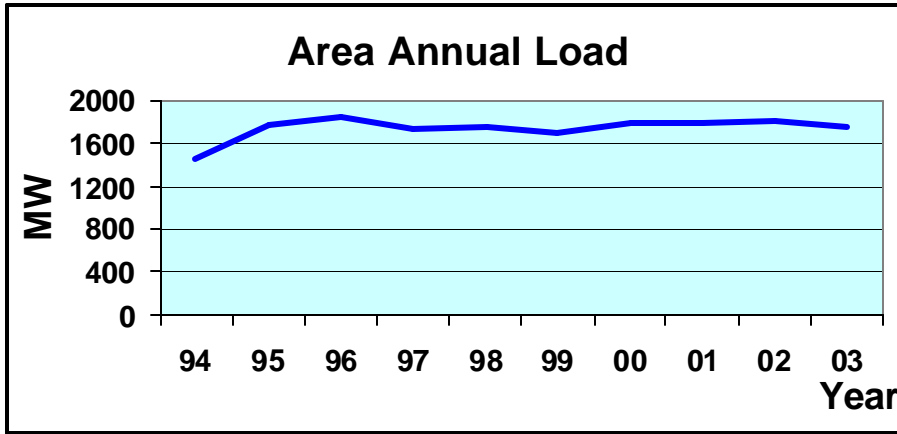
Figure A.2.27 – Area 27 Annual Load
