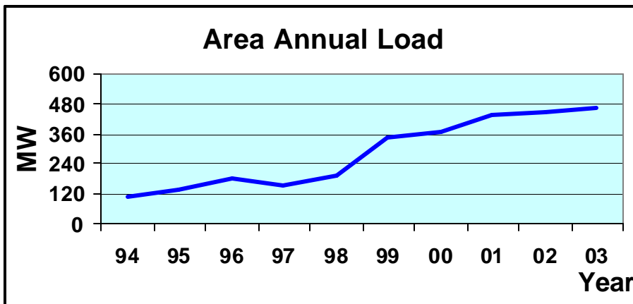
Figure A.2.26 – Area 26 Annual Load
