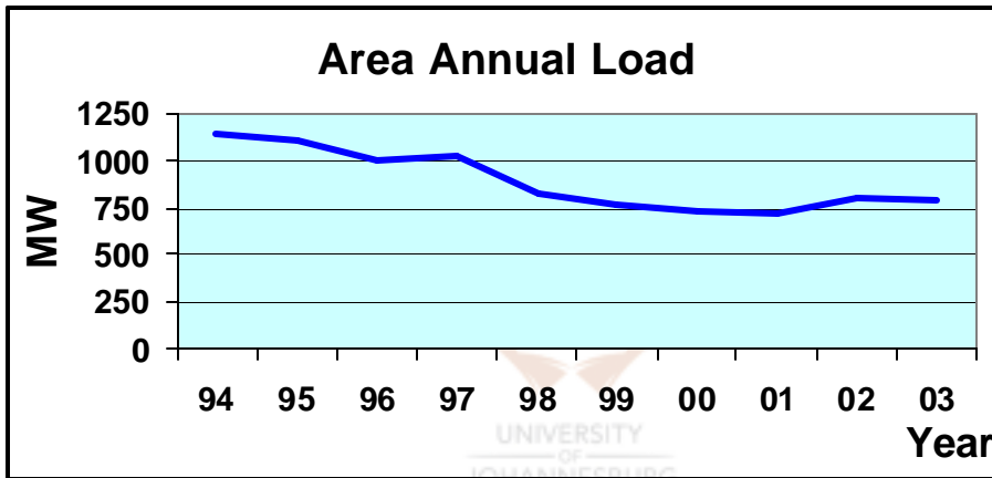
Figure A.2.25 – Area 25 Annual Load
