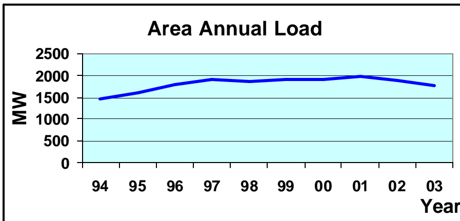
Figure A.2.5– Area 5 Annual Load
