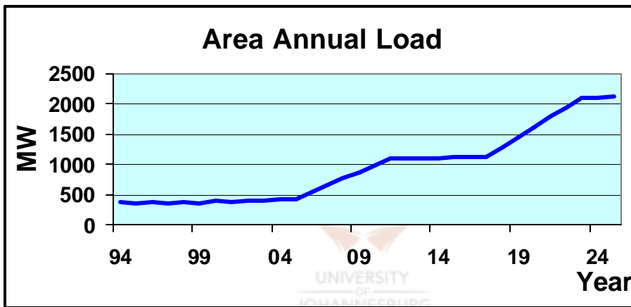
Figure A.2.28 – Area 9 Annual and Forecast Load
