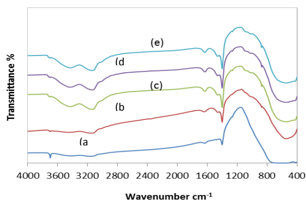
Fig. 1 FTIR spectra for (a) dried catalyst; (b) catalyst calcined at 500^\circ\text{C} ; (c) catalyst calcined at 600^\circ\text{C} ; (d) catalyst calcined at 700^\circ\text{C} and (e) catalyst calcined at 800^\circ\text{C}
