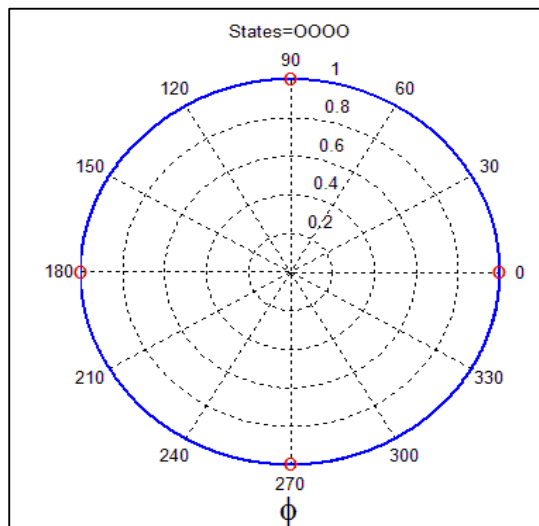
Fig. 2: Omnidirectional configuration resulting when all 4 parasitic elements are open-circuited.
