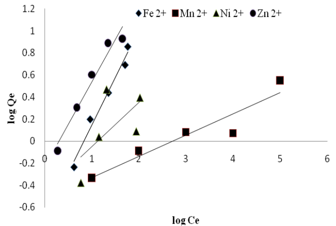
Fig. 4 Freundlich isotherm for metal removal by Clinoptilolite zeolite
