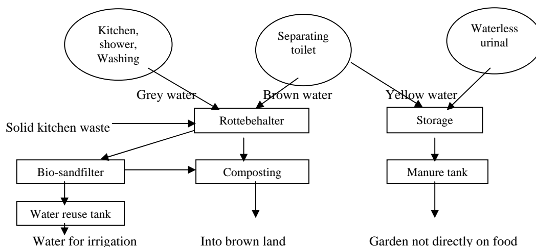
Fig. 3 Components of ecological sanitation with composting chamber
