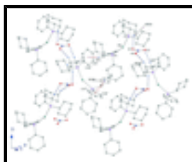
Fig. 2. A perspective of (I) where C—H \cdots O and C—H \cdots\pi intermolecular interactions are shown in dashed lines [Symmetry codes: (i) -x+1, y-1/2, -z+1; (ii) -x+2, -y-1/2, -z+2].
