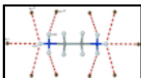
Fig. 3. : Close-up view of (I) viewed down the b axis with a slight offset clearly showing the hydrogen-bonding interactions. Hydrogen bonds are indicated by dashed lines.
