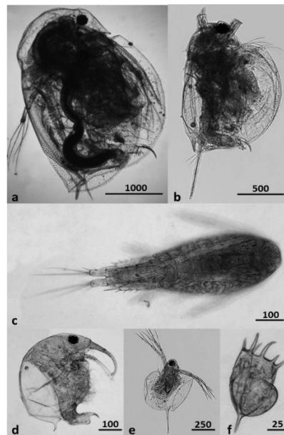
Fig. 5i (Left). Phytoplankton taxa of the lakes: a) Staurastrum pingue , b) Staurastrum quadrangulare var. attenuatum f. pentagona , c) Staurastrum bibrachiatum , d) Staurastrum laeve , e) Euastrum evolutum , f) Micrasterias radians , g) Closterium praelongum , h) Ooplanctella planoconvexa , i) Radiococcus polycoccus , j) Closterium venus . Numbers on scale bars in \mu\text{m} .
