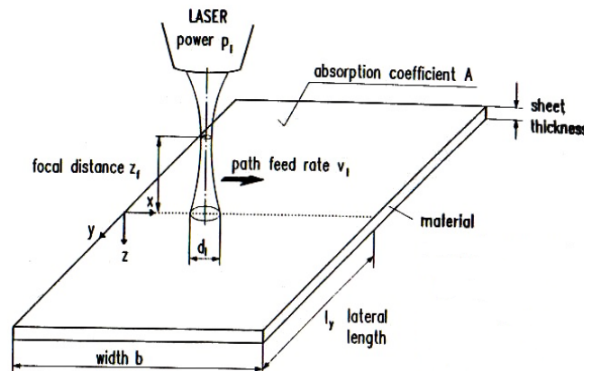
Fig. 1 Schematic of the Laser Beam Forming Process [3]
