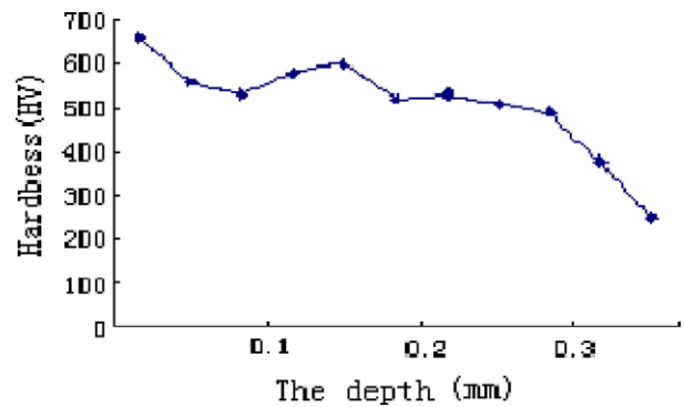
Fig. 9. The hardness.
