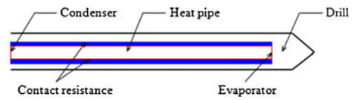
Fig. 3 Heat pipe drill fabrication
