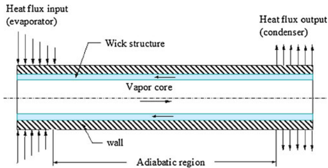
Fig. 1 Schematic of a heat pipe
