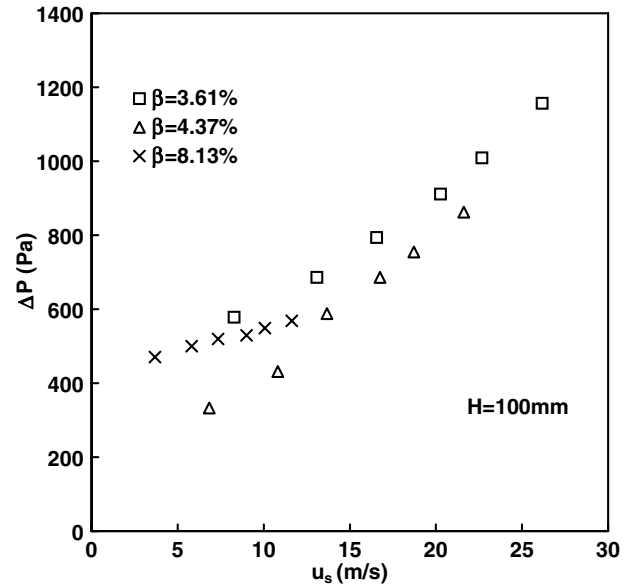
Fig. 5. Pressure drop to the air velocity at higher bubbling layer.
