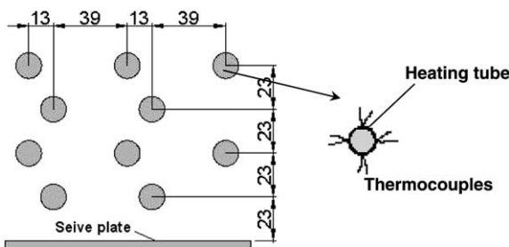
Fig. 2. Side view of the heating tube arrangement (unit: mm).
