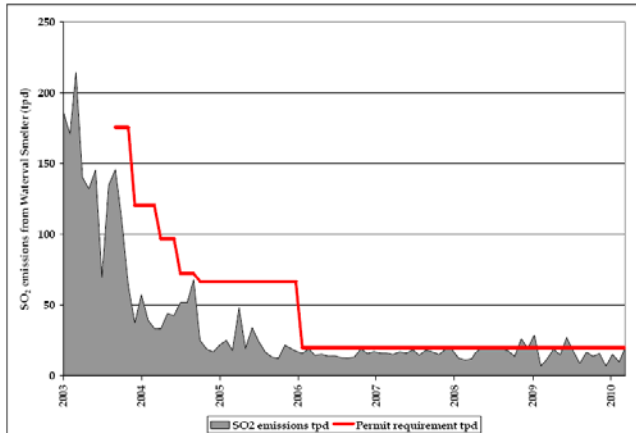
Figure 3: Decrease in \text{SO}_2 emissions at the Waterval Smelter; Source: (Hundermark et al., 2011)
