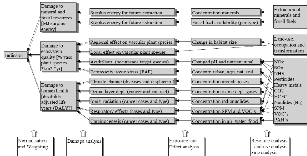
Figure 1. Graphical presentation of the Eco-indicator 99 methodology; (Pré Consultants, 2000)
