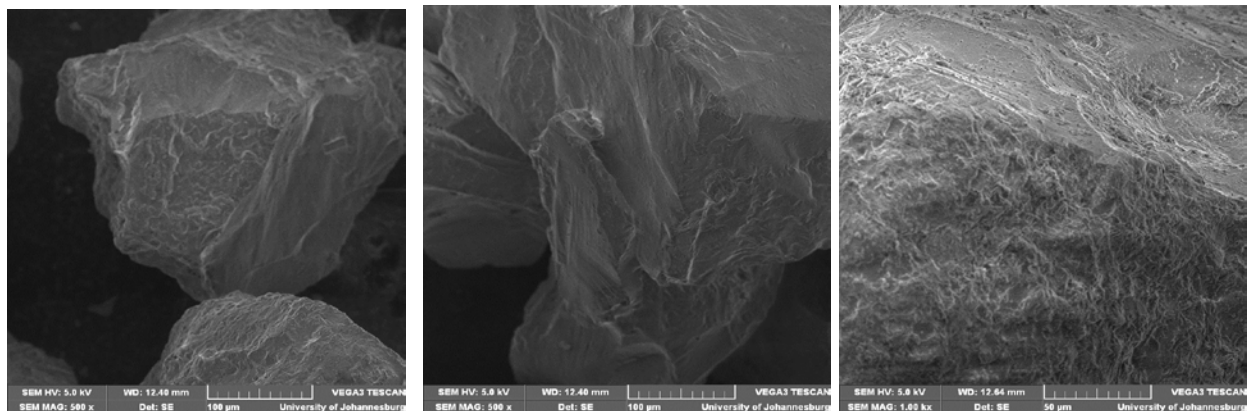
Figure 1. Moulding virgin sand surface morphology
