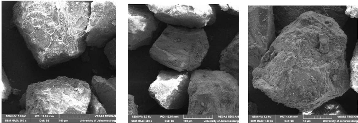
Figure 2. Waste Moulding Sand surface Morphology
