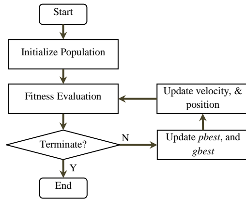
Fig. 1 Flowchart for the basic PSO
