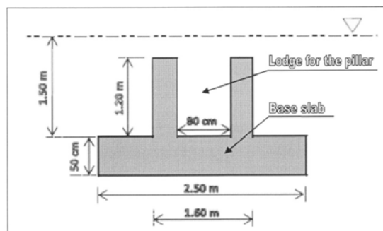
Fig. 4. Foundation plinth
