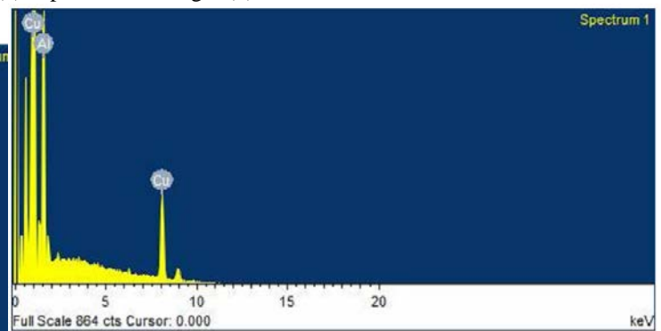
Fig. 3(b). Analysis of spectrum 1 for weld produced at 600 rpm and 150 mm/min
