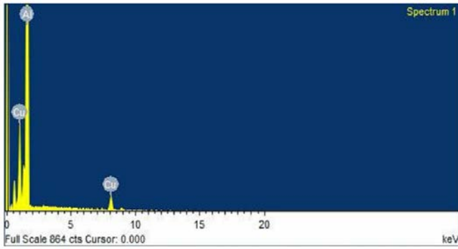
Fig. 4(b). Analysis of spectrum 1 for weld produced at 600 rpm and 300 mm/min
