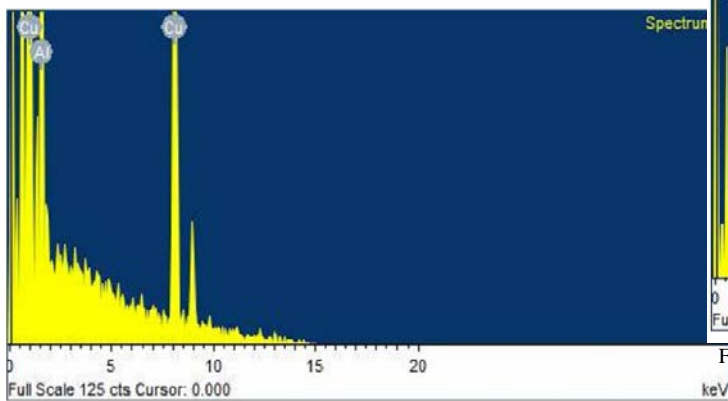
Fig. 2(b). Analysis of spectrum 1 for weld produced at 600 rpm and 50 mm/min
