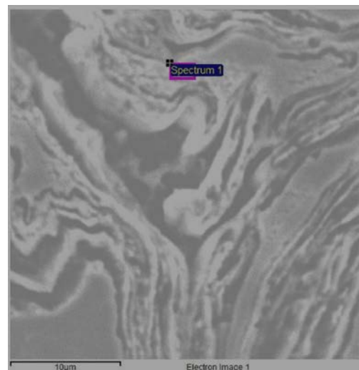
Fig. 4(a). SEM image of weld conducted at 600 rpm and 300 mm/min
