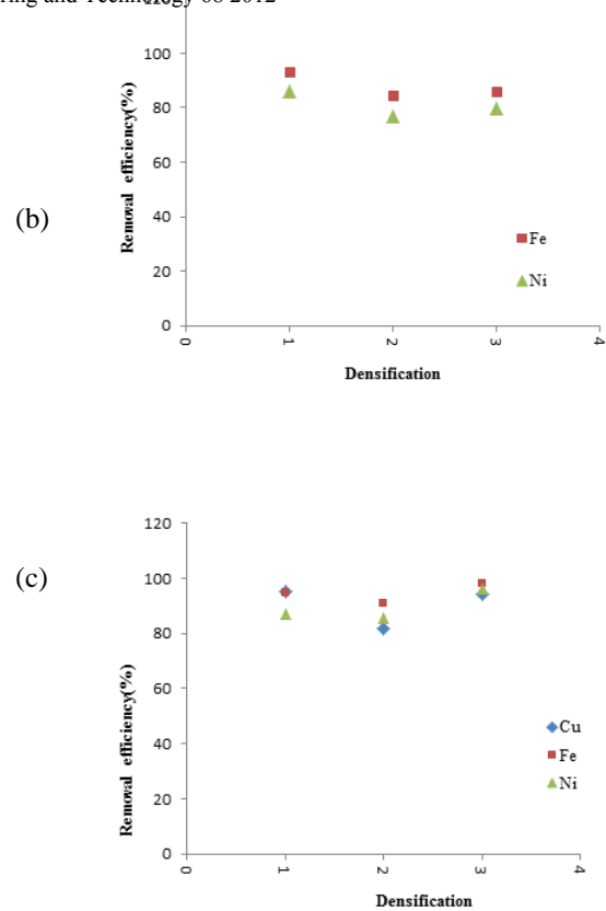
Fig. 1 Average removal efficiency of Ni, Cu and Fe (a) Ni-Cu solution (b) Ni-Fe solution and (c) Ni-Cu-Fe solution.
