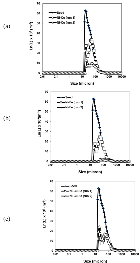
Fig. 3 Evolution of the PSD (a) Ni-Cu (b) Ni-Fe (c) Ni-Cu-Fe
