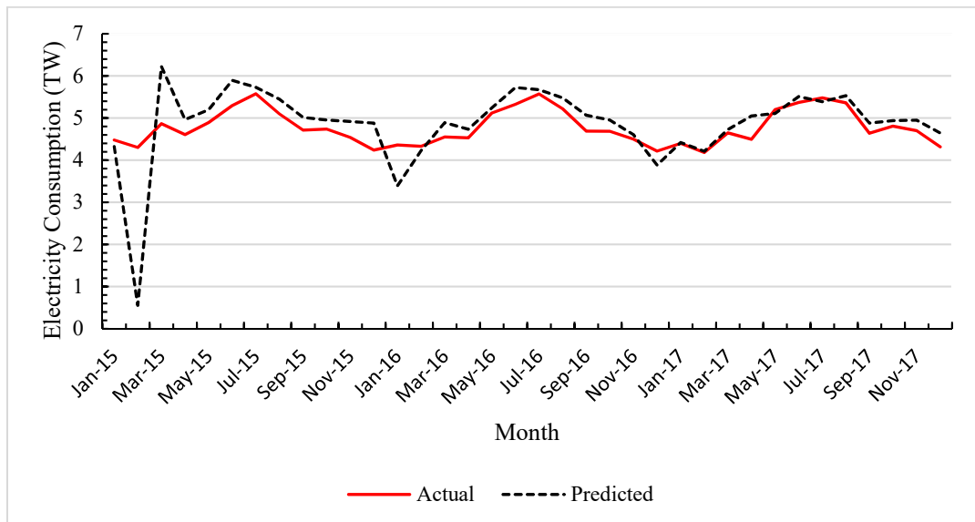
Figure 3. Prediction results for the ANFIS-FCM model at testing phase between January 2015 to Dec 2017
