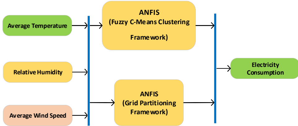
Figure 1. The forecasting model using ANFIS framework
