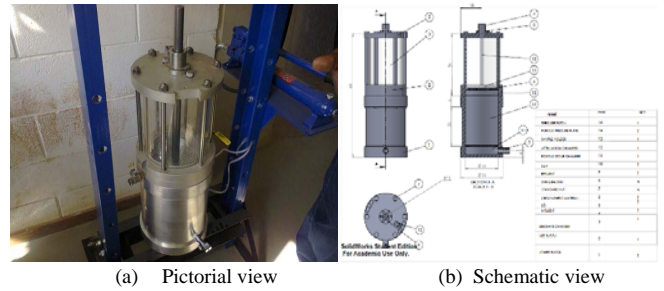
Fig. 2. (a) and (b): The small scale bespoke device used in the study
