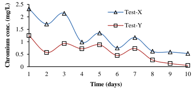
Fig. 7b. Measured chromium for tests on CDW with and without materials treated with CCA
