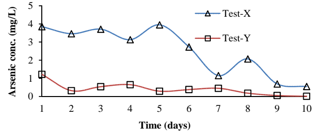
Fig. 7a. Measured arsenic for tests on CDW with and without materials treated with CCA
