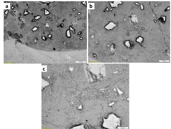
Fig. 3 2000W, 3.2 Ti-6Al-4V+ B 4 C+BN showing strong bond strength between the coated layer and the substrate with a little crack defect
