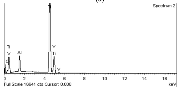
Figure 3 (a) Ti6Al4V powder, 3(b) the analysis of Ti6Al4V powder
