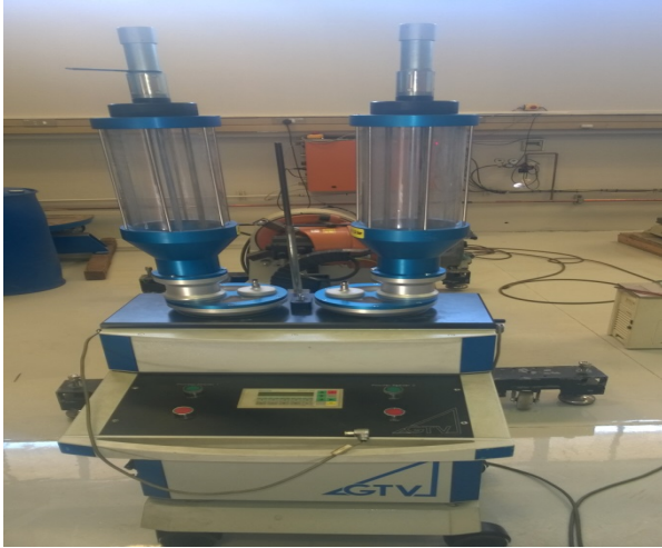
Figure 2: Powder feeder
