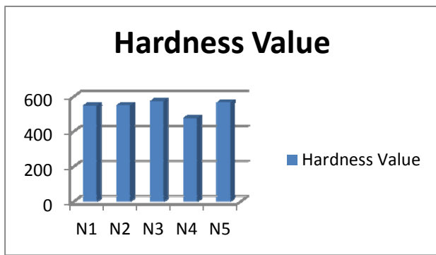
Figure 5: Micro-hardness distributions in the composite coatings
