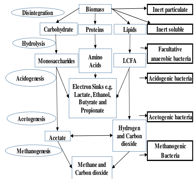
Fig. 1. Degradation steps of the anaerobic digestion process.
