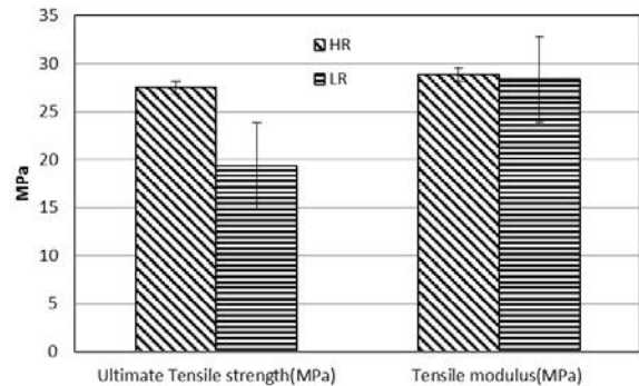
Figure 10 - Effect of resin transfer rate
