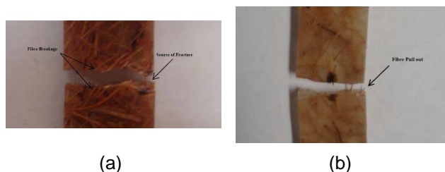
Figure 6 - Sample fractured specimens (a) Flat (b) Fiber pull out
