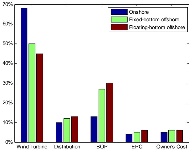
Figure -5 Component cost distribution for wind power plant [39]
