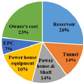
Figure -3 Cost component distribution for pumped hydro storage
