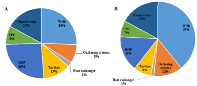
Figure -2 Cost distribution for geothermal plant, A- Hydrothermal, B- Enhanced Geothermal plant
