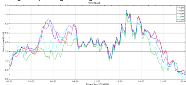
Figure -9 Intermittent wind speed profile for Alexander Bay, South Africa [61]
