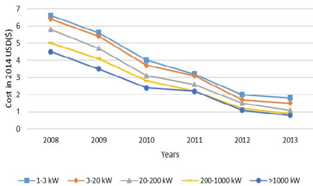
Figure -8 Decline in solar PV module prices between 2008 and 2013 [58]
