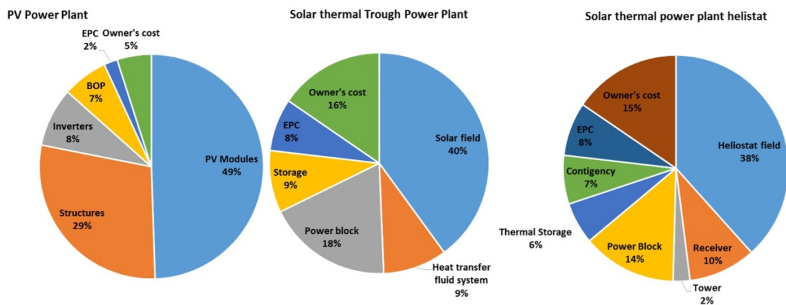
Figure -4 Component cost distribution for solar power plant [39]
