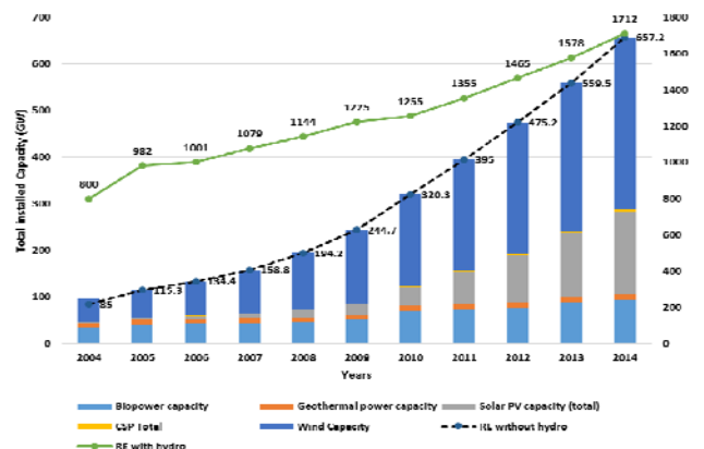
Figure -7 Cumulative electricity installed capacity for renewable energy sources [40, 54]
