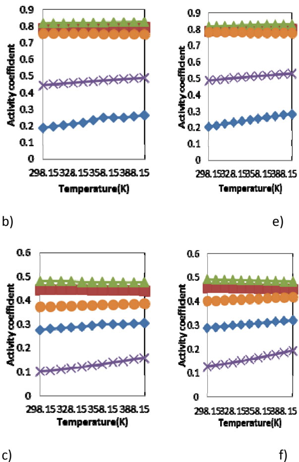
Fig.2. Variation of activity coefficients with temperature for the Alkane family in Methyl Stearate for a) Original UNIFAC; b) Modified UNIFAC Bastos; c) Modified UNIFAC Larsen; Methyl Oleate for d) Original UNIFAC; e) Modified UNIFAC Bastos; f) Modified UNIFAC Larsen
