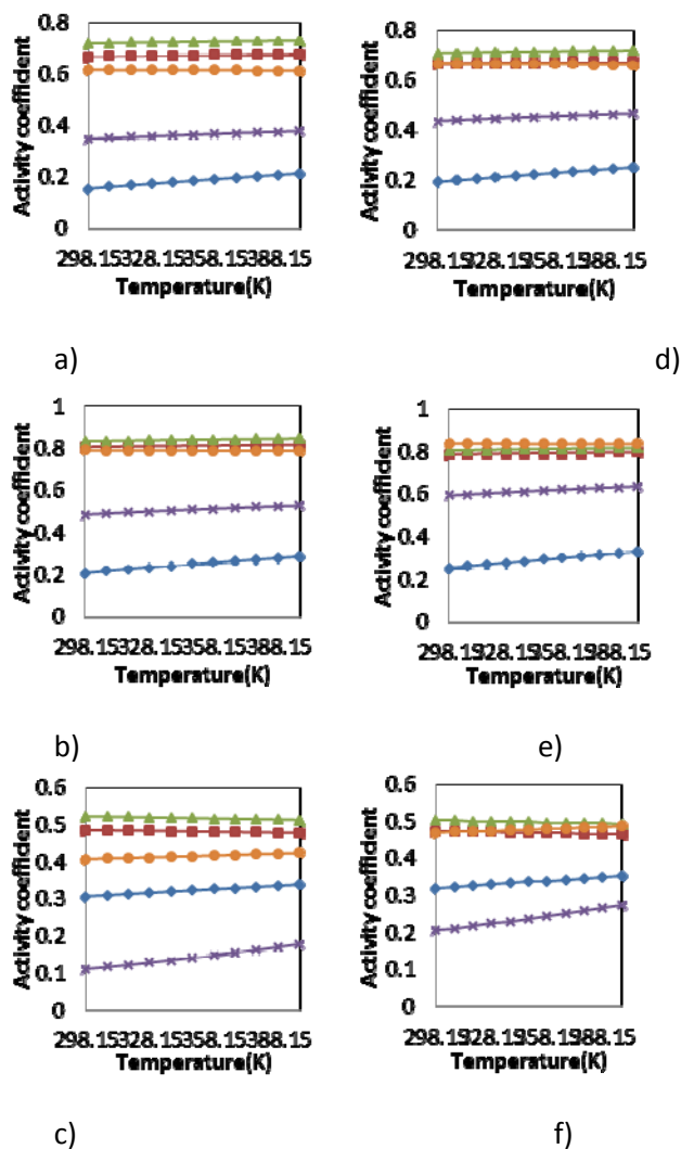
Fig.1. Variation of activity coefficients with temperature for the Alkane family in Methyl Palmitate for a) Original UNIFAC; b) Modified UNIFAC Bastos; c) Modified UNIFAC Larsen; Methyl Linolenate for d) Original UNIFAC; e) Modified UNIFAC Bastos; f) Modified UNIFAC Larsen
