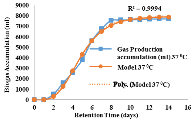
Fig. 3. Biogas Prediction using Modified Gompertz model for pig waste/grass.
