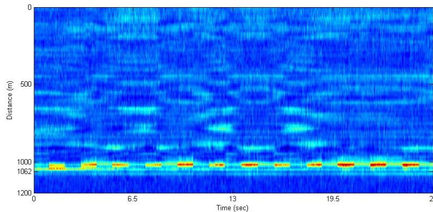
Fig.6. Waterfall plot for the full length of the fiber. An amplitude of the cross-correlation is presented in pseudo-colors; red corresponds to maximum signal amplitude.
