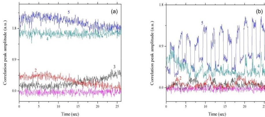
Fig.5. Time variation of cross-correlation amplitudes measured at 4 different positions along the fiber(traces 2-5); (a) without an external perturbation; (b) a perturbation was applied at the distance of 1016 meters. Trace 1 represents the background level of the system noise, trace 2: measured at the distance of 500m; 3: at distance 710 m; 4: at distance 1050 m; 5: at distance 1016m where perturbation was applied. An array of FBG interferometers were formed in the fiber section from 1015 to 1070 meters).
