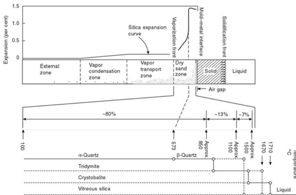
Figure 4 - Structure of the heated surface of a greensand mould against a steel casting; and the forms of silica (after Sosman 1927) with solid lines denoting stable states and broken lines denoting unstable states. [4]
