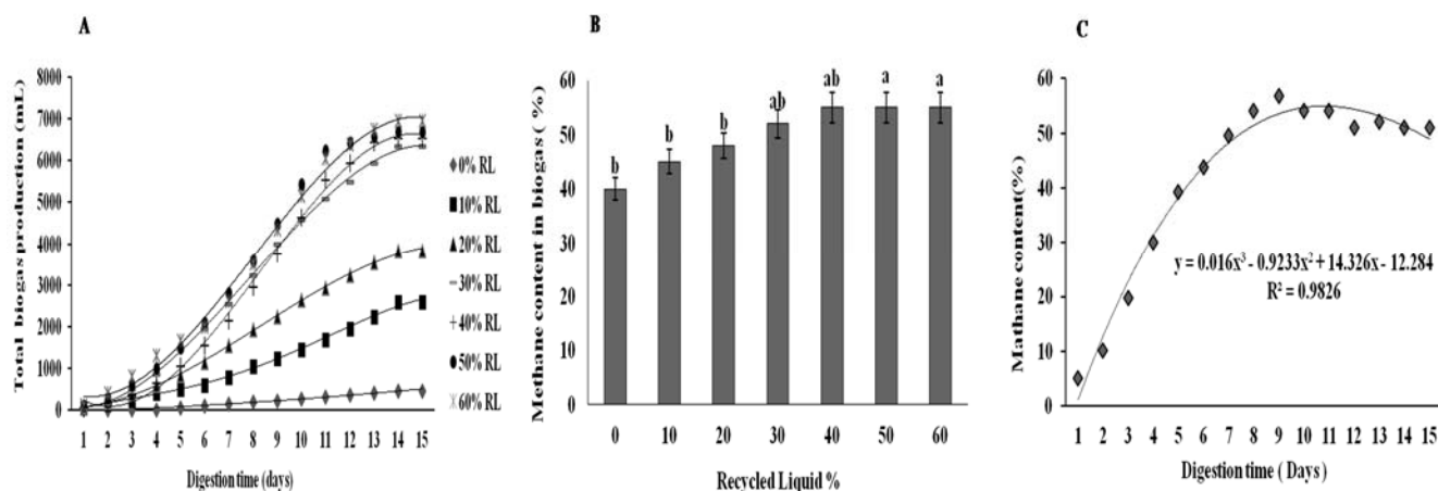
Fig. 2 Total biogas production (A), methane content (B), methane content with respect to time (C) obtained during anaerobic digestion of lawn grass with recycled liquid digestate. b is methane content range from 40-45%,
