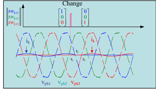
Fig. 3 Switching mechanism
