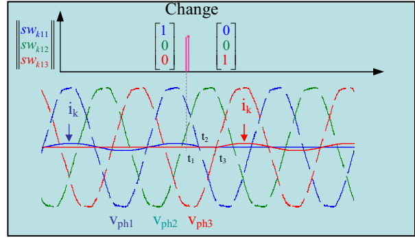
Fig. 3 Switching mechanism
