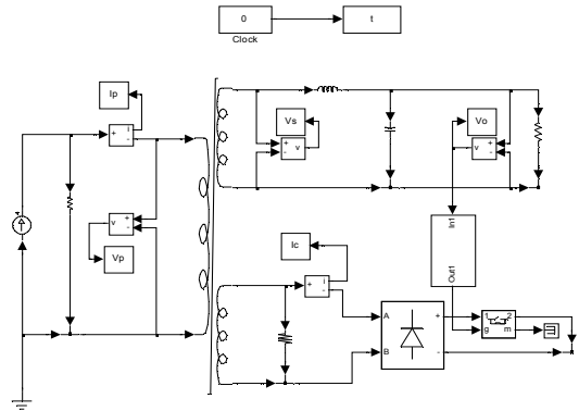
Fig. 4. Simulation model
