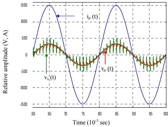
Fig. 6. Output voltage for 1 kHz switching frequency and k = 20\%
