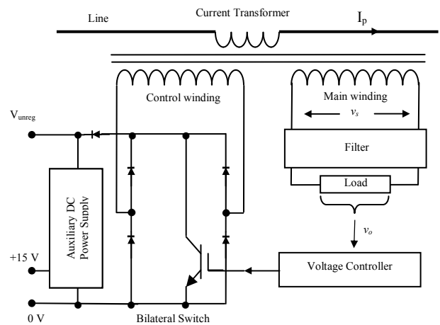
Fig. 2. Basic circuit
