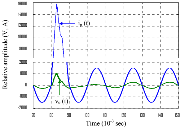
Fig. 10. Impact of a big input current transient
