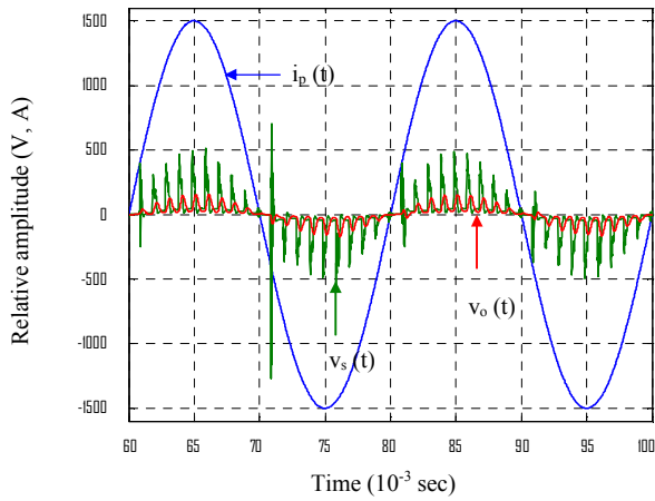
Fig. 5. Output voltage for 1 kHz switching frequency and k = 80\%
