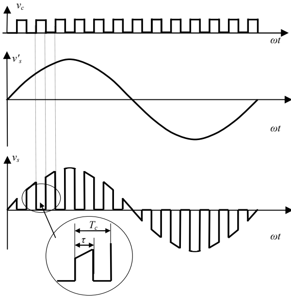
Fig. 3. Secondary voltage generation
