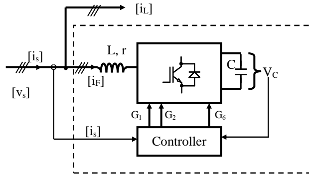
Fig. 1: Active power filter in parallel with a partially balanced feeder
