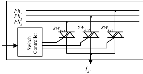
Fig. 2. Switch selector.
