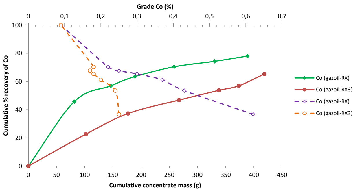
Fig. 8 Comparison between Co recoveries and grades obtained with the mixture gazoil-rinkalore RX and the mixture gazoil-rinkalore RX3
