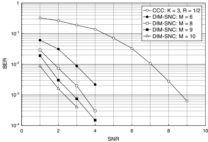
Fig. 4. Hard decision decoding with QPSK/OFDM and AWGN.
