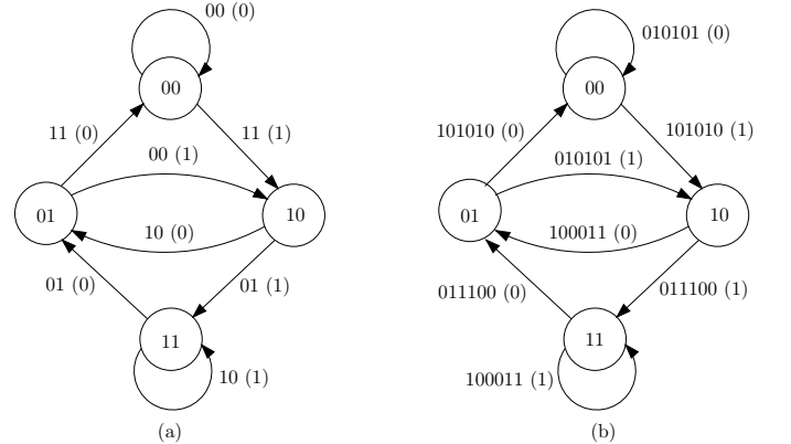
Fig. 3. State systems for the (a) convolutional code and (b) DPM-SN code.
