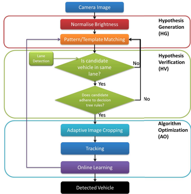
Figure 1. Flowchart of the vehicle detection algorithm design.
