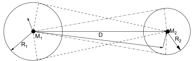
Figure 1: Uniformly distributed circular scattering regions surrounding mobile nodes modeling mobile-to-mobile propagation environment.
