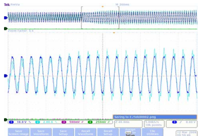
Figure 17. Response of the machine to sudden load change to 9.5Nm
