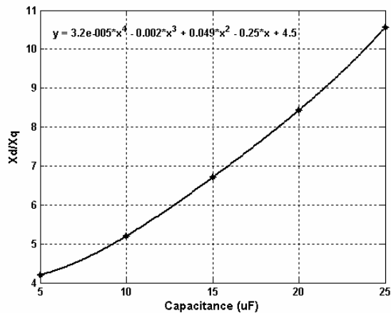
Figure 7. Variation of measured saliency ratio with the Capacitance injected
