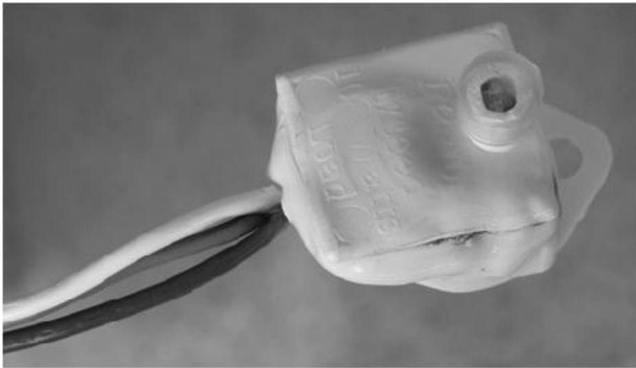
Figure 10: Switch Overheated by CFL Load
