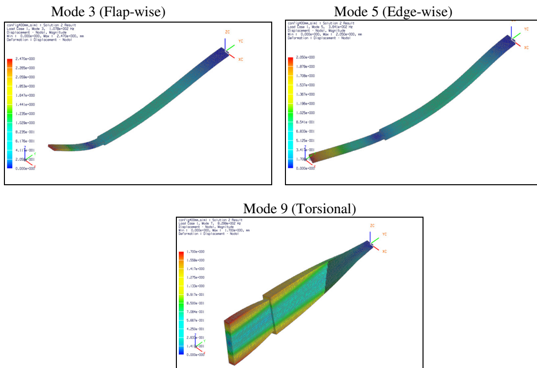
Figure 6: Flap-wise, edge-wise and torsional deflection for configuration 5
