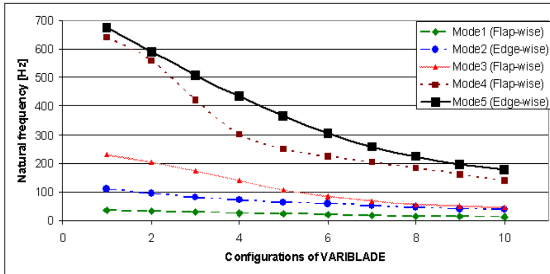
Figure 9: Natural frequencies
