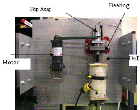
Figure 8 - Experimental setup
