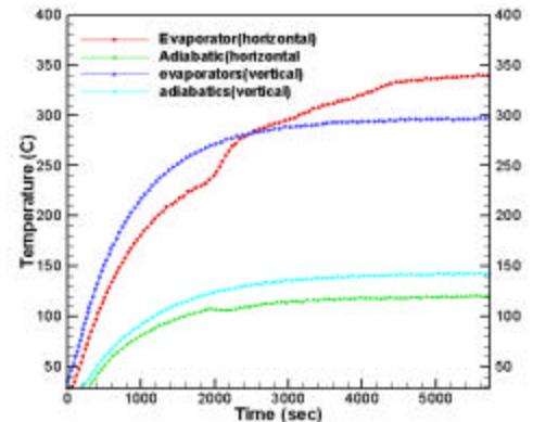
Figure 14 - Effect of different orientation on drill with heat pipe under 1000 rpm operation speed
