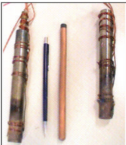
Figure 2 - Steel solid cylinder with and without a heat pipe
