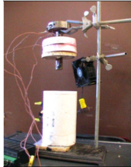
Figure 3 - Experimental Setup
