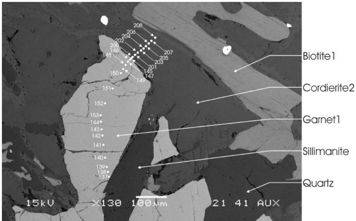
Figure A5.3: Position of microprobe points in profile 10 across garnet and cordierite.
