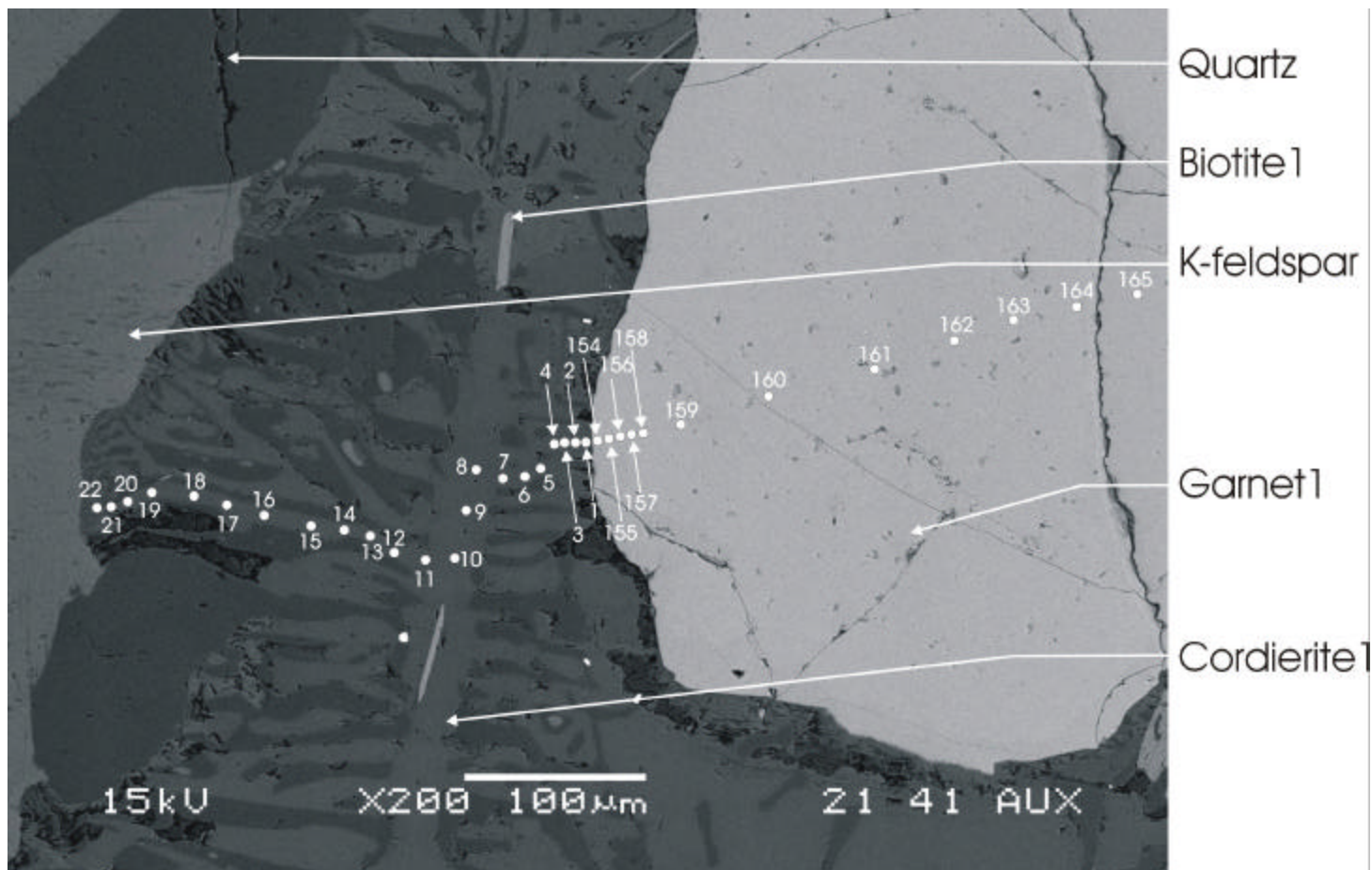
Figure A5.2: Position of microprobe points in profile 8 across garnet and contacting cordierite
