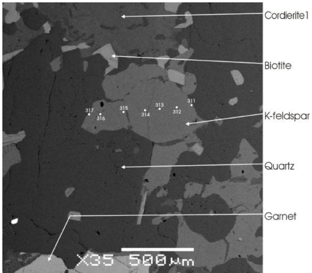
Figure A5.4: Position of microprobe points in profile 9 across K-feldspar
