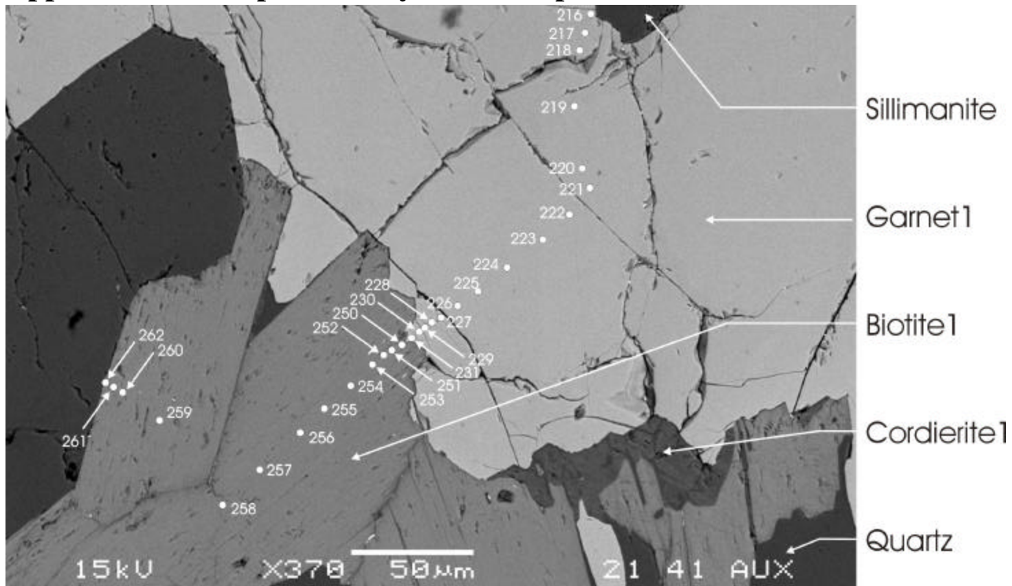
Figure A5.1: Position of microprobe points in profile 7 across biotite and contacting garnet.
