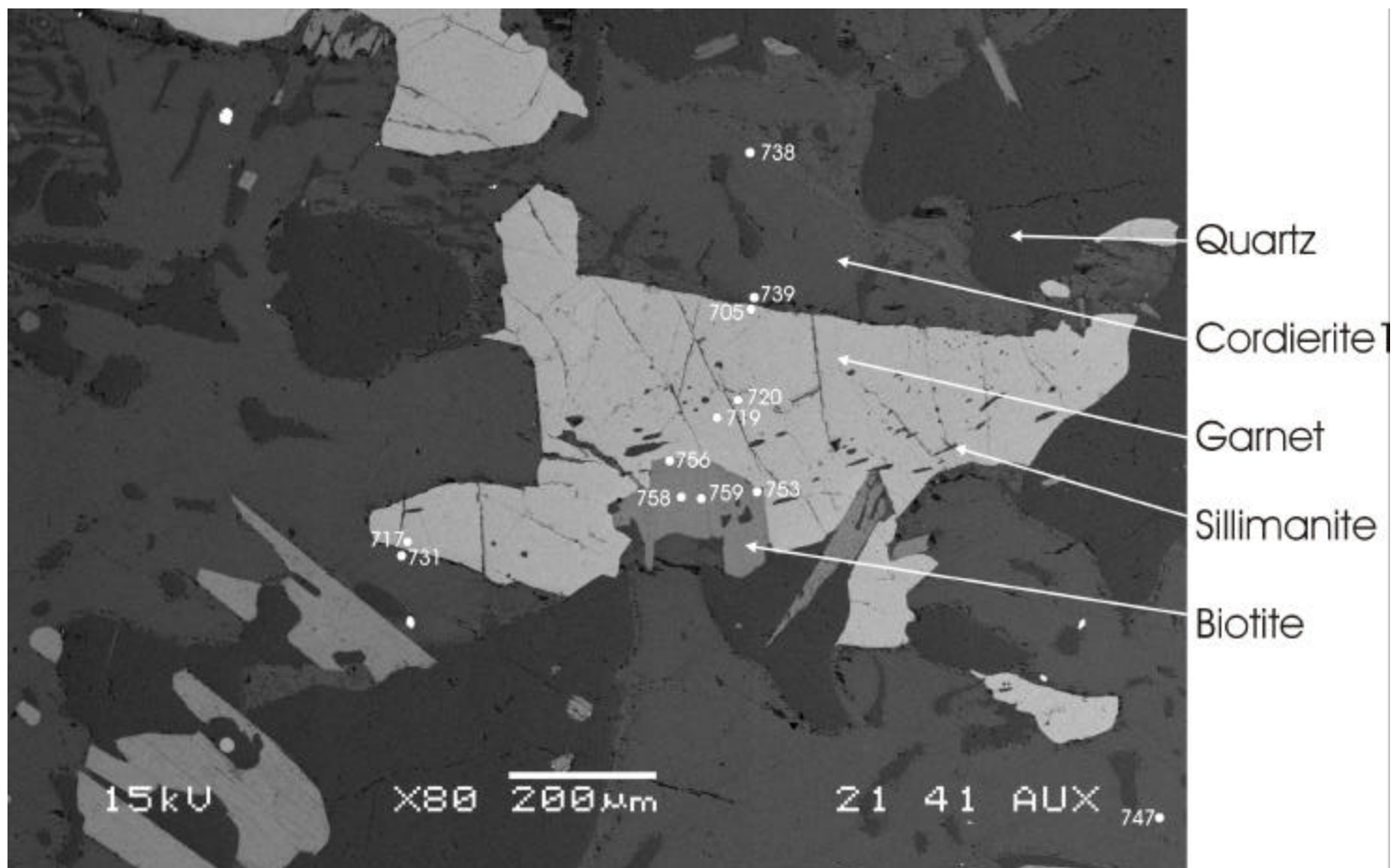
Figure A5.6: Position of microprobe points used for thermobarometry
