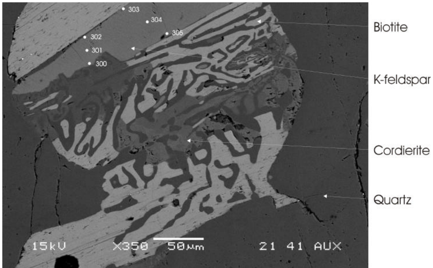
Figure A5.5: Position of microprobe points across K-feldspar used for thermobarometry.
