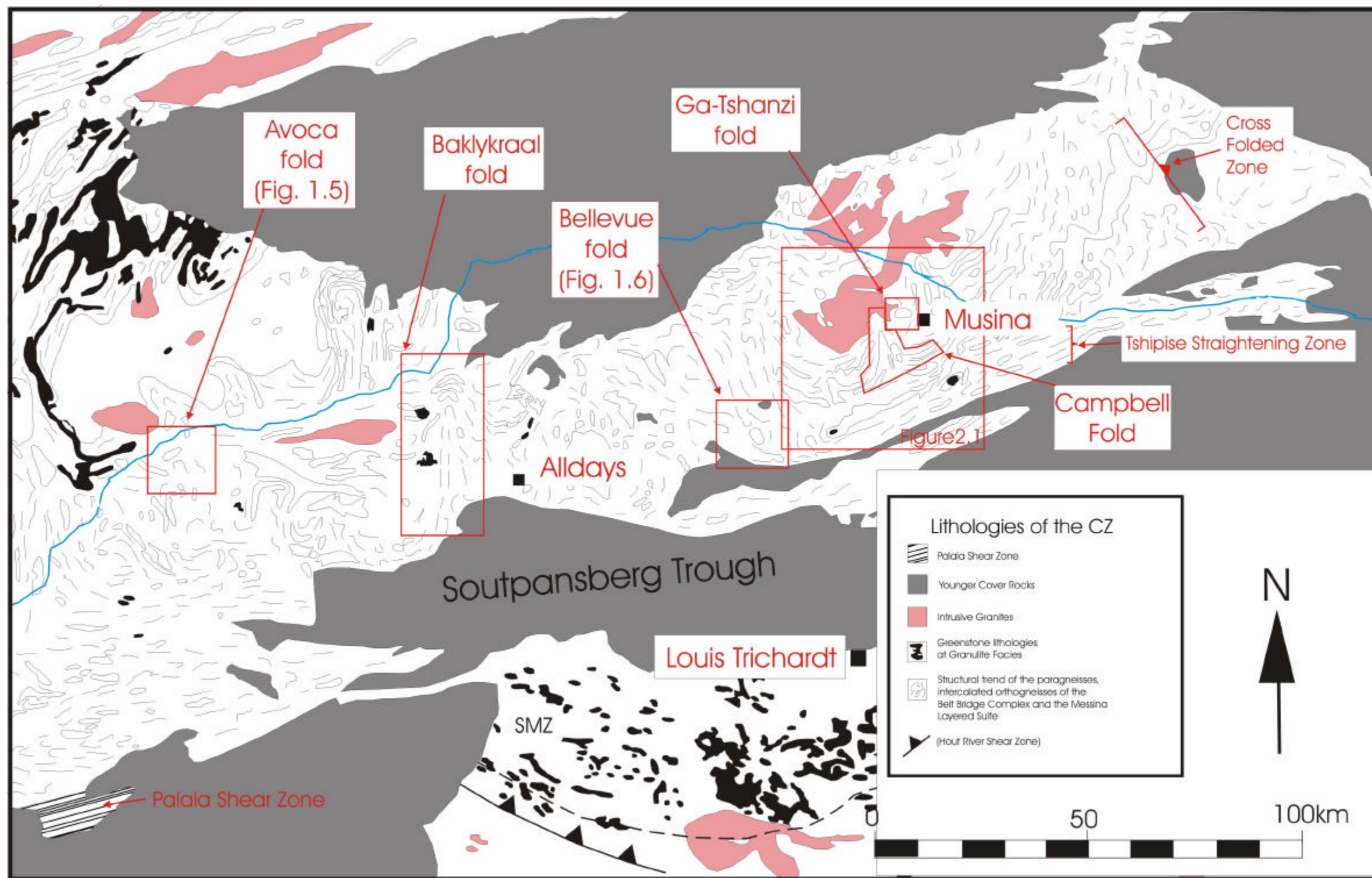
Figure 1.3: The regional geology of the Central Zone (Modified from Van Reenen et al., 1995).
