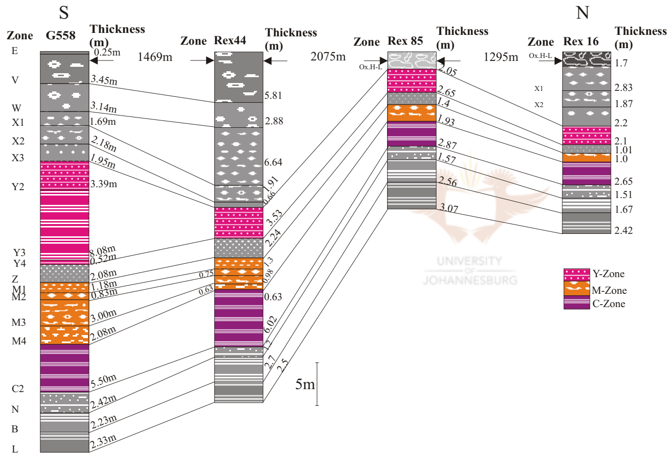
Figure 2.10 North-south section of the Lower Manganese Body through the study area using selected drill cores (ref. Fig. 2.6). Dramatic thinning between Rex 44 and Rex 85 is evident. The overall thinning can be mainly attributed to thinning of the M and C-zones, i.e., the lower part of the economic zone. E - Supergene manganese ore logged by Preston (2001), Ox. L - Oxidised hematite lutite
