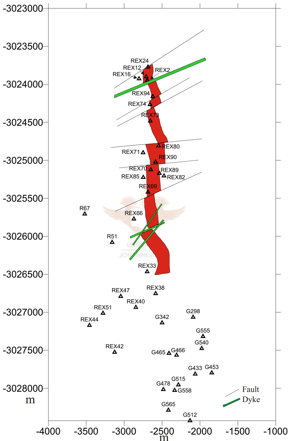
Figure 2.5 Map illustrating the position of the studied boreholes (REX), previous boreholes, marked by G (Preston, 2001), the suboutcrop of the Lower manganese ore bed against the Kalahari Formation and main structures present in the study area.
