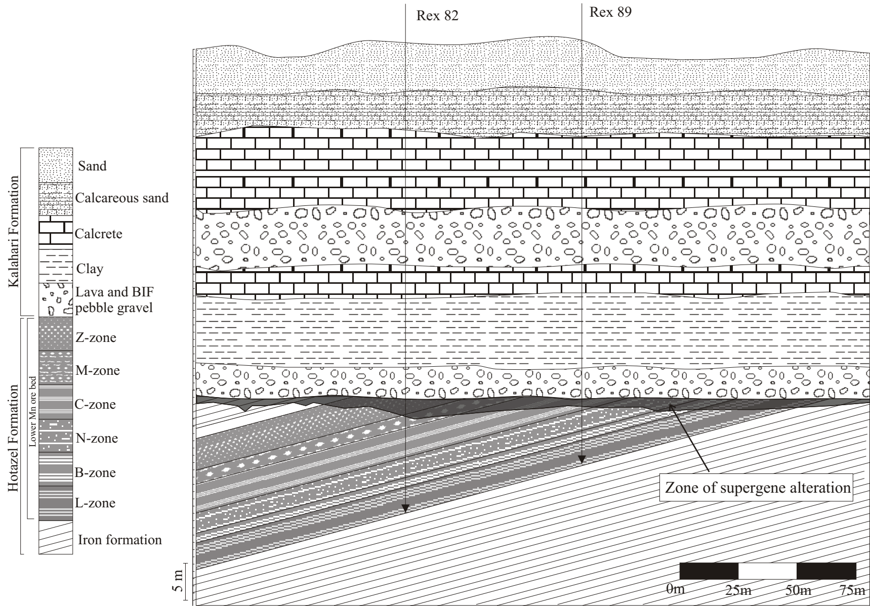
Figure 2.6. Schematic illustration of the suboutcrop of the Hotazel Formation against the Kalahari Formation and associated supergene alteration in the study area.
