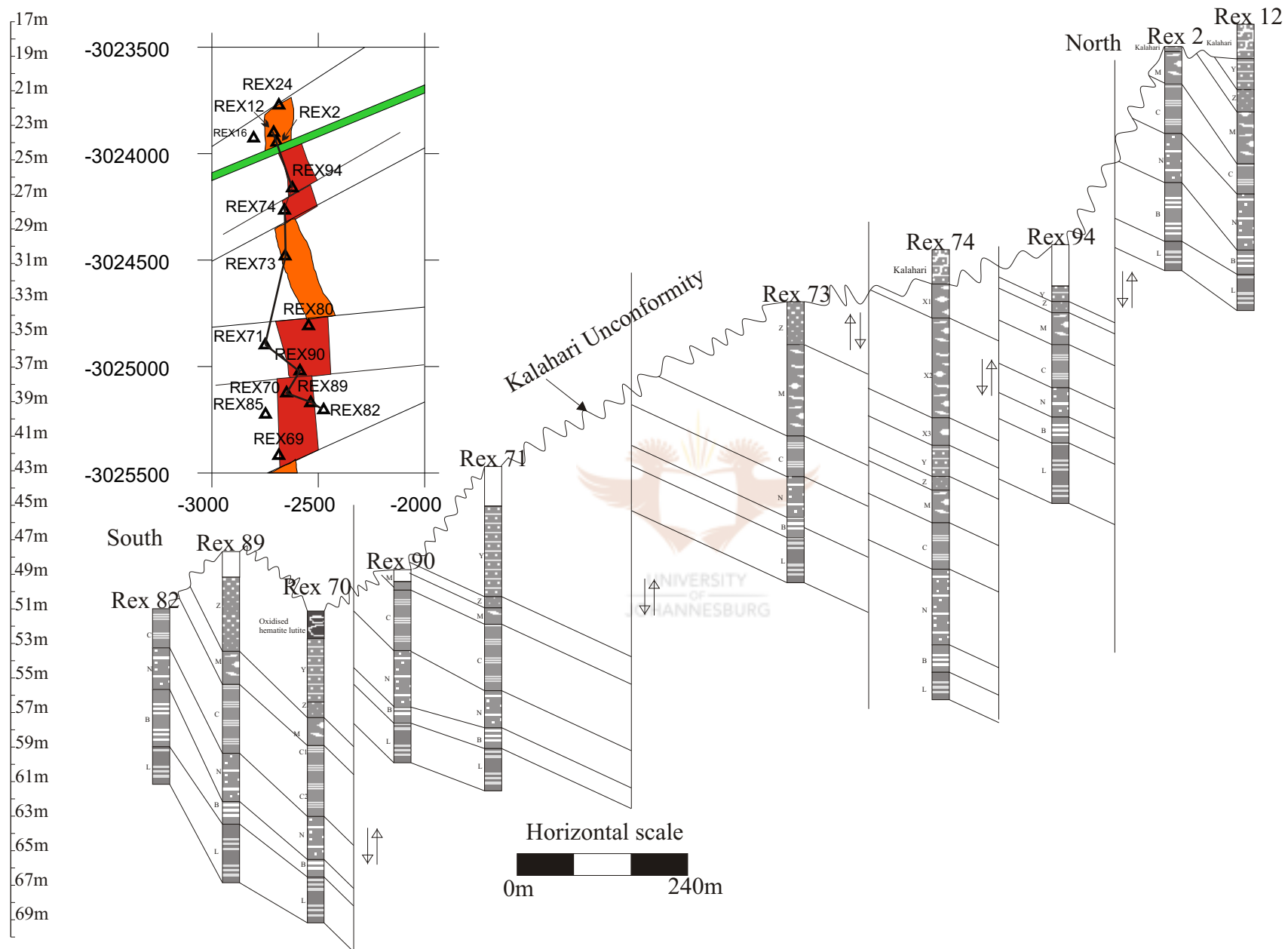
Figure 2.7. North-south section to illustrate the influence of the Kalahari Unconformity on the presence of lithostratigraphic zones along the eastern suboutcrop perimeter of the Lower Mn Body. Note that the black coloured blocks mark supergene altered Mn ore, intersected by percussion holes as logged by S.J. Van der Merwe for Samancor Manganese, Hotazel.
