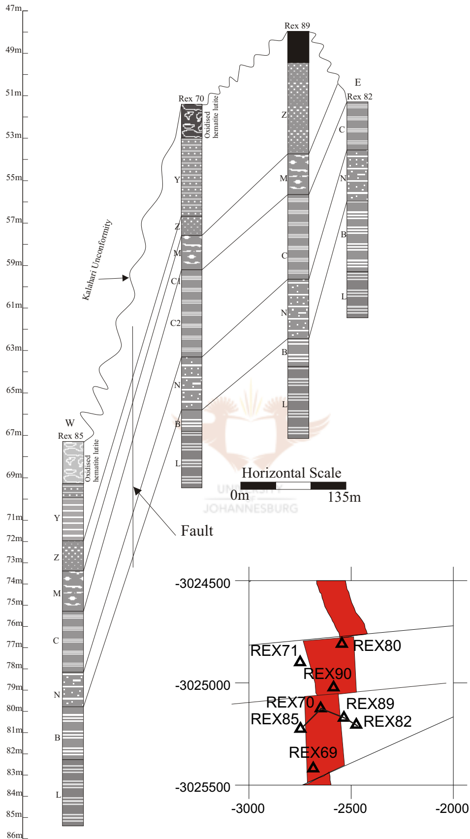
Figure 2.8. East-west section to illustrate the influence of the Kalahari Unconformity on the presence of lithostratigraphic zones along the eastern suboutcrop perimeter of the Lower Mn Body. Note that the black blocks define supergene altered Mn ore as logged by S.J. Van ver Merwe from percussion drill holes.
