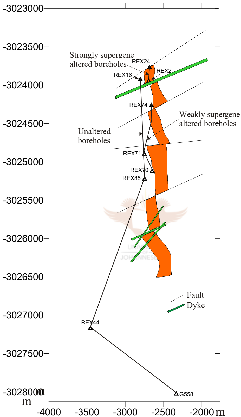
Figure 4.1. Map illustrating the exact localities of the drill cores sampled for geochemical investigations. Unaltered braunite lutite is represented by Rex 16, Rex 85 and Rex 44; weakly supergene altered braunite lutite samples were obtained from Rex 70, Rex 71 and Rex 74; and strongly supergene altered braunite lutite samples are from Rex 2 and Rex 24. Please note that a complete set of geochemical data is also available for drill core G558 in the Mamatwan Mine area (Preston, 2001).
